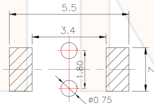
PCB Lavout
